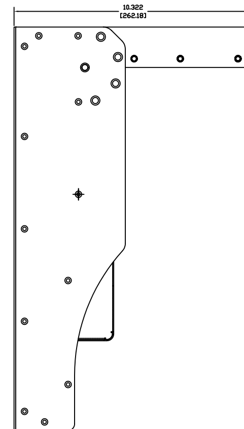
SIDE VIEW (UNFOLDED)
